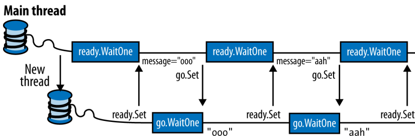
Figure 22-2. Two-way signaling
